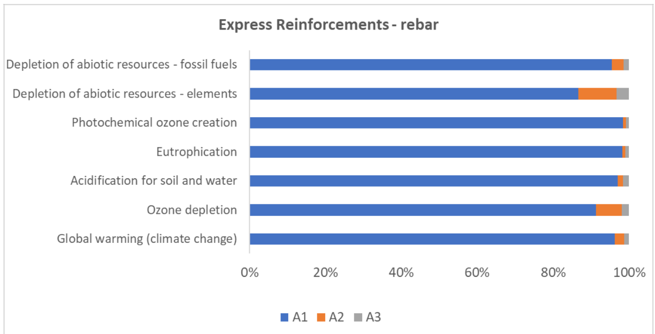
Figure 4 – Cradle- to-gate LCIA hotspots for Express Reinforcements cut and bent steel rebar product
