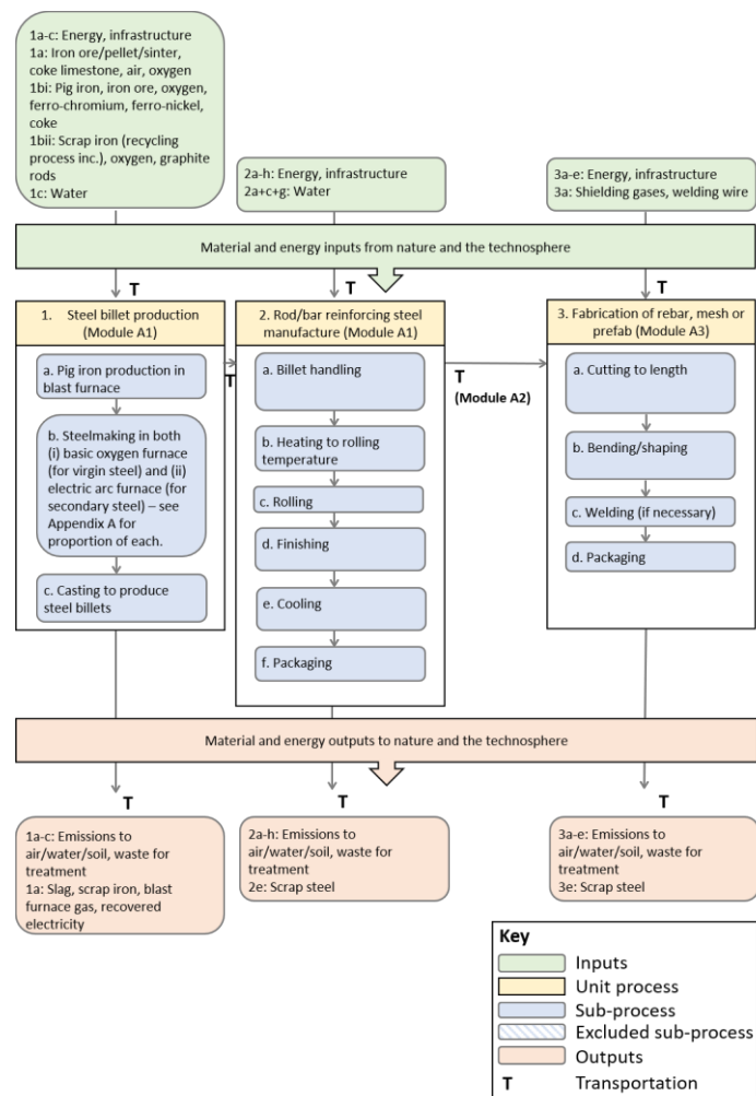
Figure 3 – Process flow diagram
